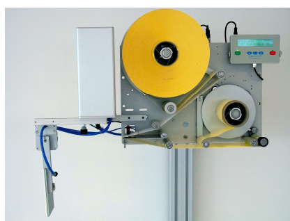
With swing arm
